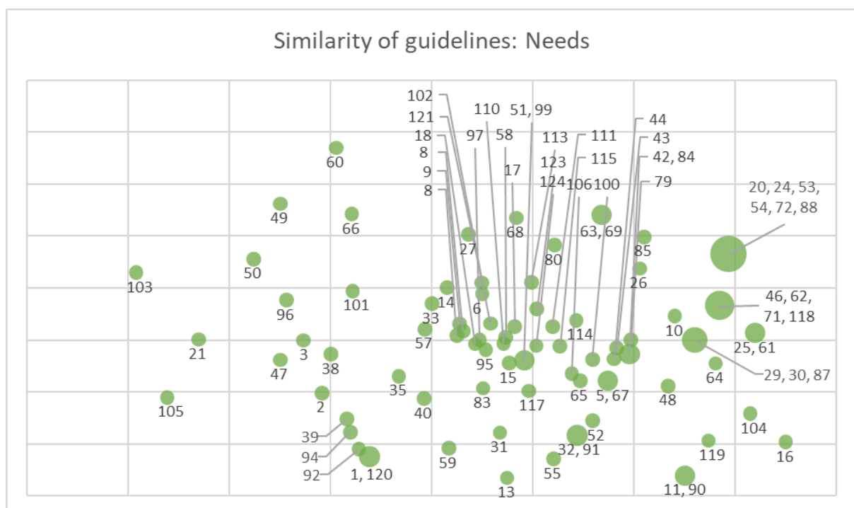
Figure 7: Similarity of guidelines matched with needs from the regions visualized with MDS in a 2D format. Bray-Curtis similarity. 2D stress: 0,18
