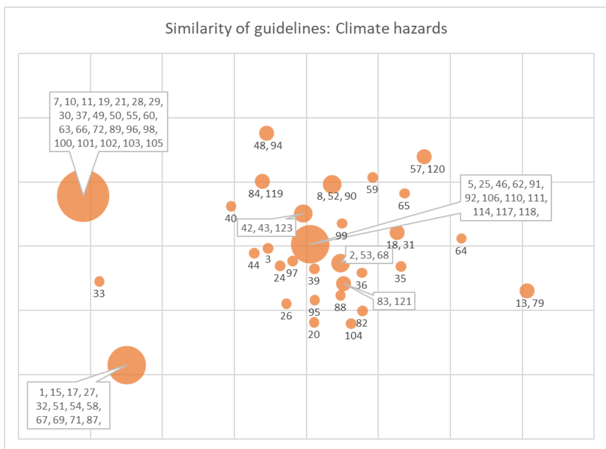
Figure 6. Similarity of guidelines matched with climate hazards visualized with MDS in a 2D format. Bray-Curtis similarity. 2D stress: 0,04
