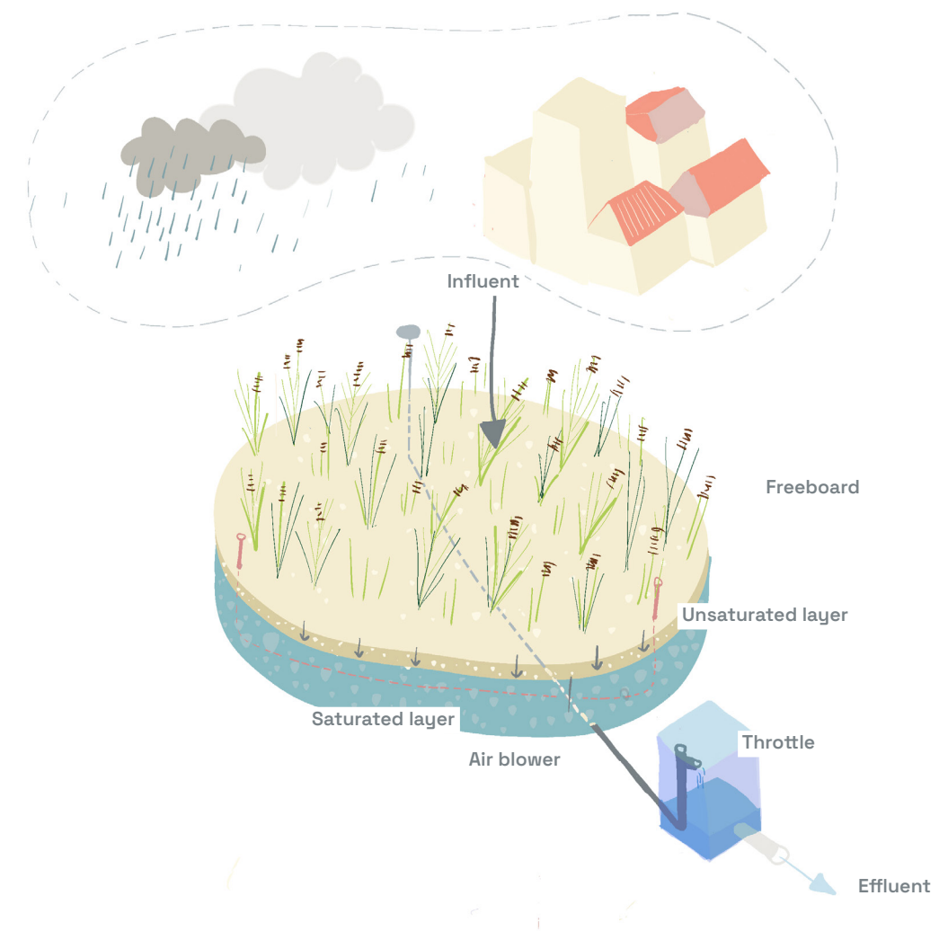
Figure 2.4.1 Typical representation of an aerated vertical flow treatment wetland for CSO.
