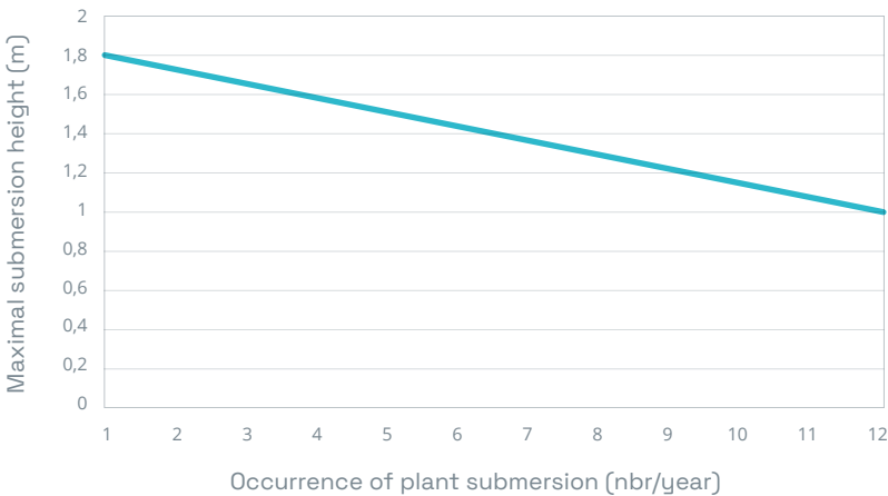
Figure 2.3.4 Permitted submersion height based on the occurrence of rain events (Molle et al., 2014)
