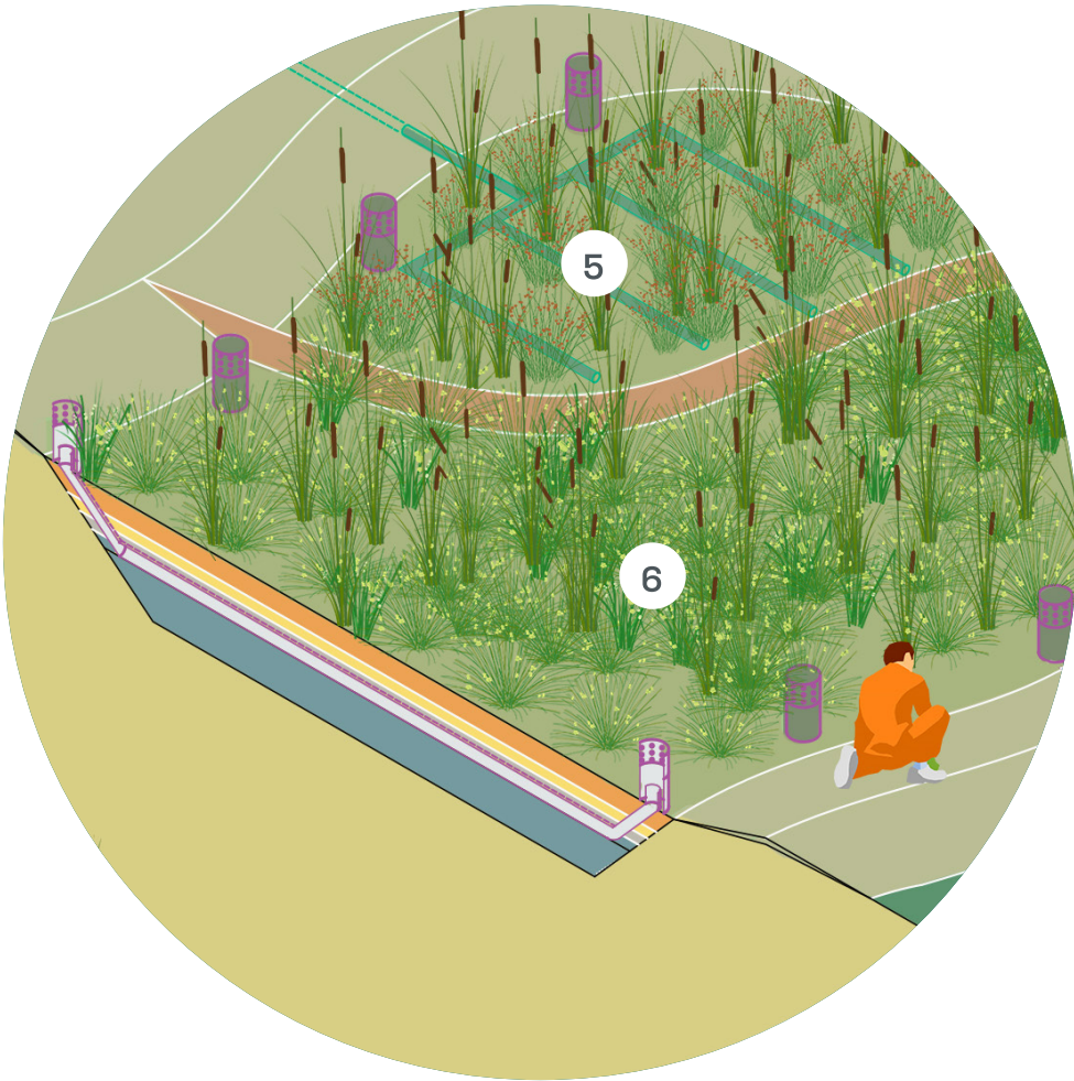
Figure 2.3.12 Cross section of the treatment wetland, Algeciras Urban Real Lab (NICE project).
