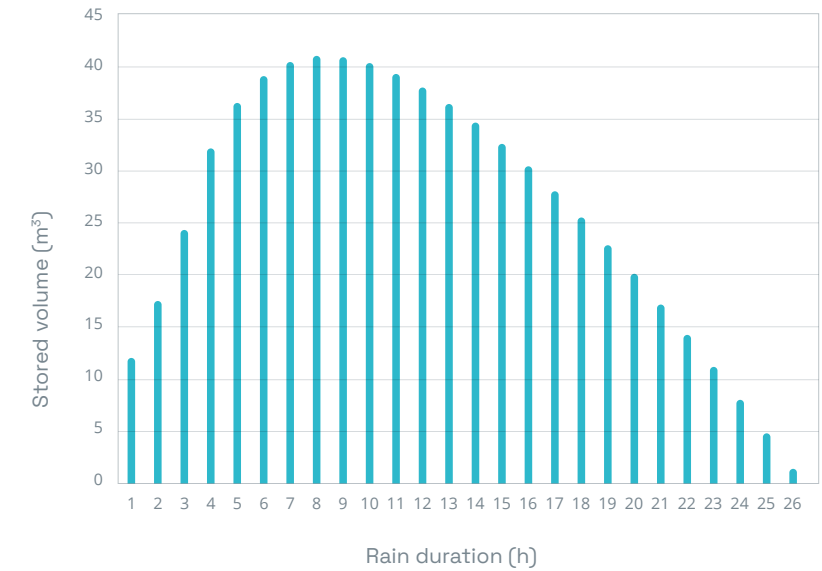
Figure 2.3.9 Storage capacity as a function of the rain duration for a 20 mm/d rain event (design rain).
