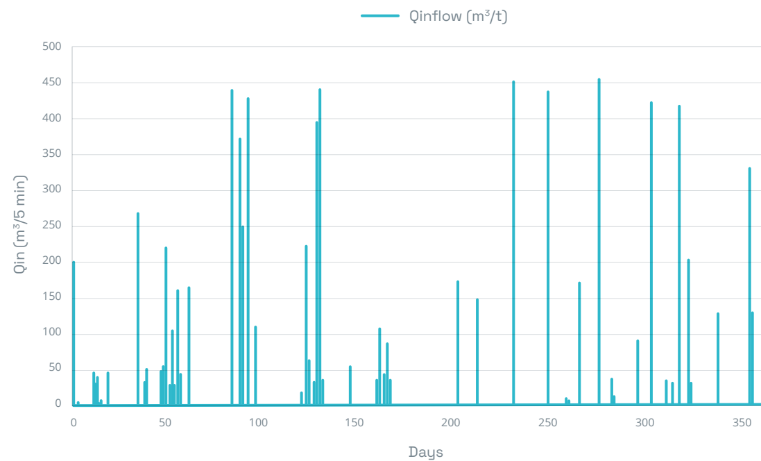
Figure 2.4.2 Annual overflow data series used for design.
